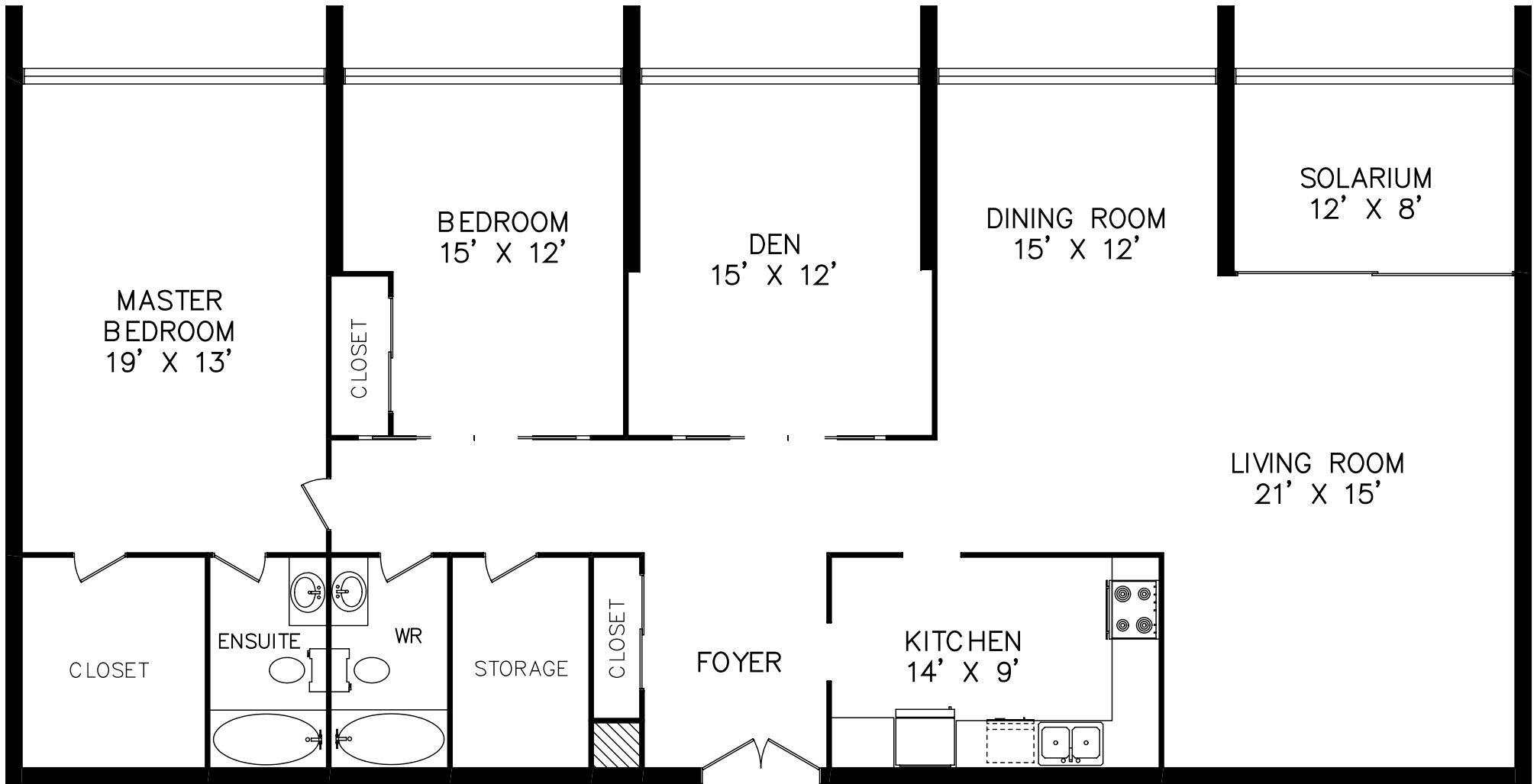
OLD MILL TOWERS TWO BEDROOM SUITE + DEN "C"
